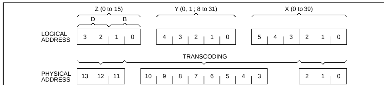
Figure 11 : Logical to Physical Address Transcoding Performed On-chip
