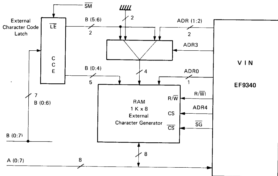
FIGURE 8 — ADDING AN EXTERNAL CHARACTER GENERATOR
