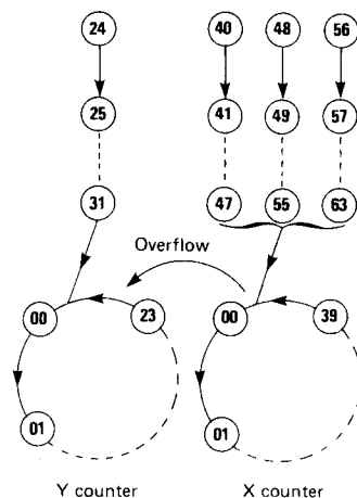
STATE DIAGRAM
