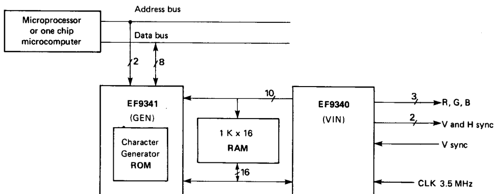
FIGURE 1 - TYPICAL DISPLAY UNIT
